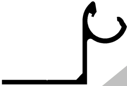
26004 Remate Lateral Exterior
